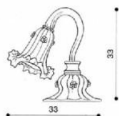
VIVALDI.P1L 1xE14 40W
