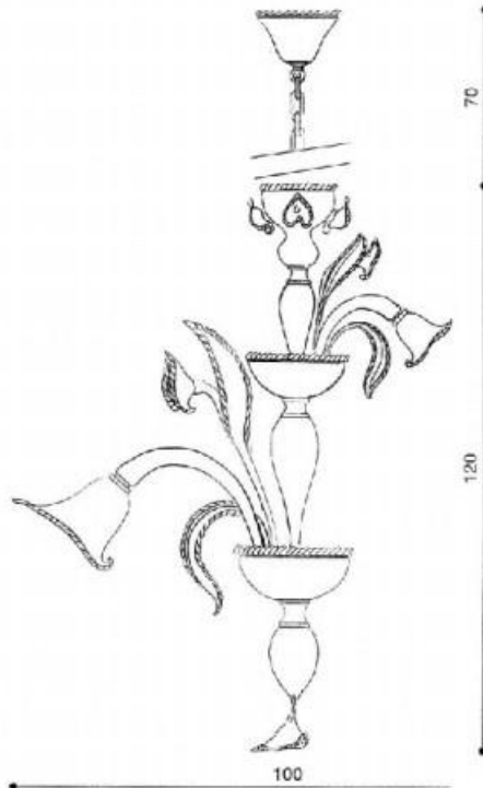
ALBINONI.S 8+4 12 FIAMME xE14 40W
